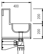
D4: Thermoformed with upstand - for wall mounted taps
