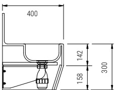
D2: Thermoformed with splashback and removable access panel - for deck mounted taps
