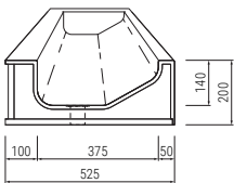
T1: Sloping thermoformed - for deck mounted taps
