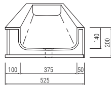
T3: Thermoformed - for deck mounted taps
