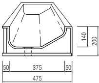
T2: Sloping thermoformed - for wall mounted taps
