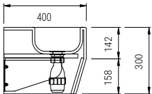
D3: Thermoformed with removable access panel - for deck mounted taps
