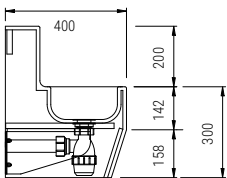
D1: Thermoformed with upstand and removable access panel - for wall mounted taps
