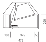
T5: Concealed waste - for deck mounted taps
