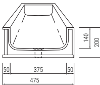
T4: Thermoformed - for wall mounted taps
