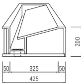
T6: Concealed waste - for wall mounted taps
