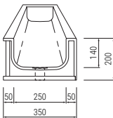
T4S: Slim thermoformed - for wall mounted taps
