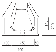
T3S: Slim thermoformed - for deck mounted taps
