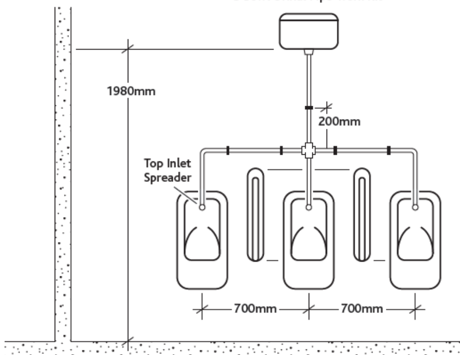
3 Bowl Urinal Pipe-work Kit
