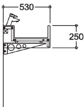
SCTR102: For Deck Mounted Taps
